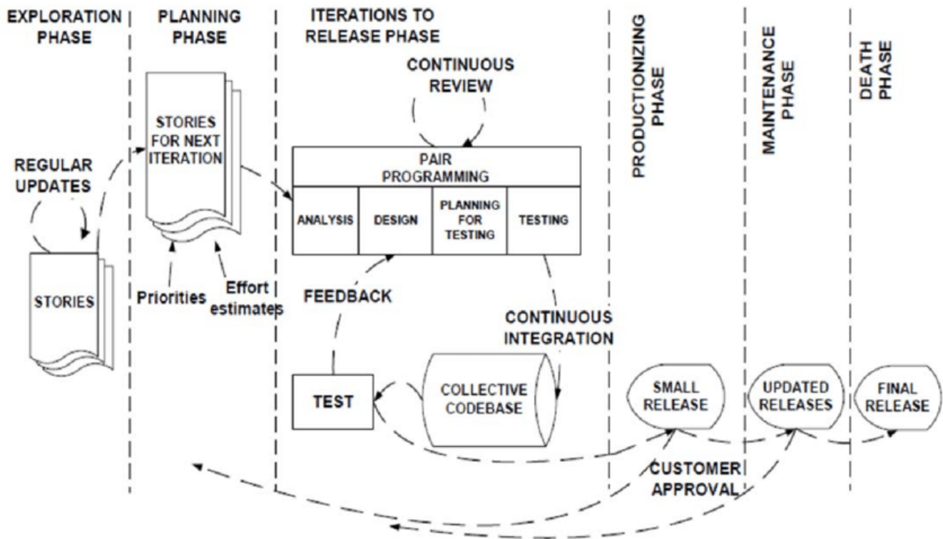
Fig 1: Shows Extreme Programming (XP) process model
