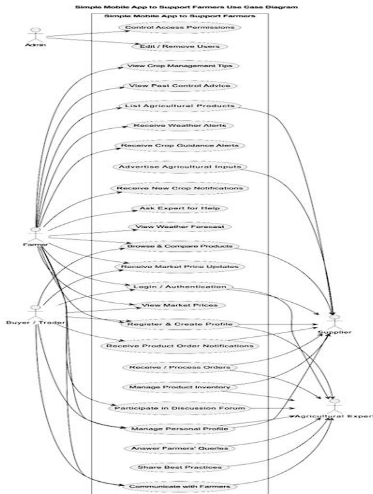
Fig 3: Shows use case diagram
